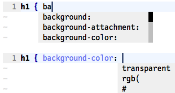
Figure 5—Omni-completion of CSS properties and values
