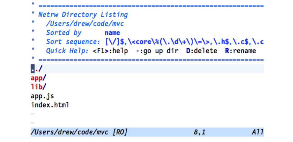
Figure 2—netrw—Vim’s “native” file explorer
