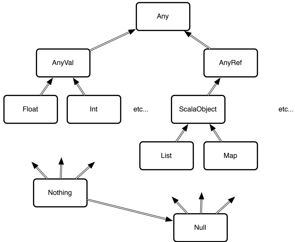
Figure 6—Any and Nothing
