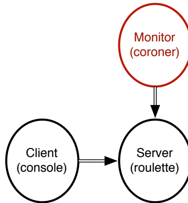
Figure 8—Adding monitoring
