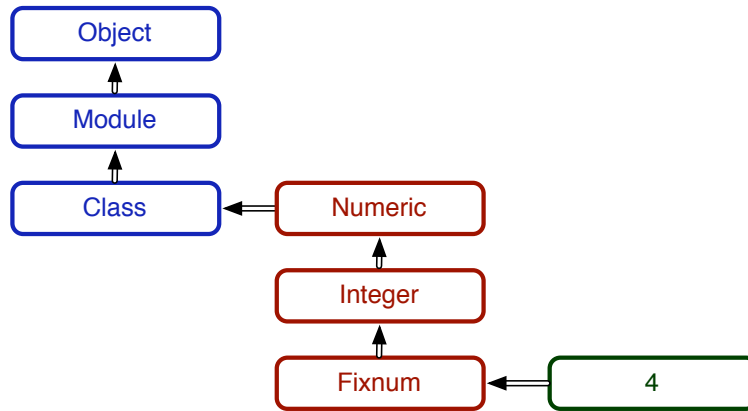
Figure 1—Ruby metamodel
