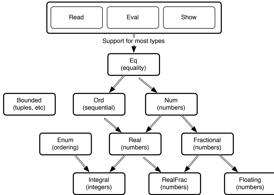
Figure 9—Important Haskell classes
