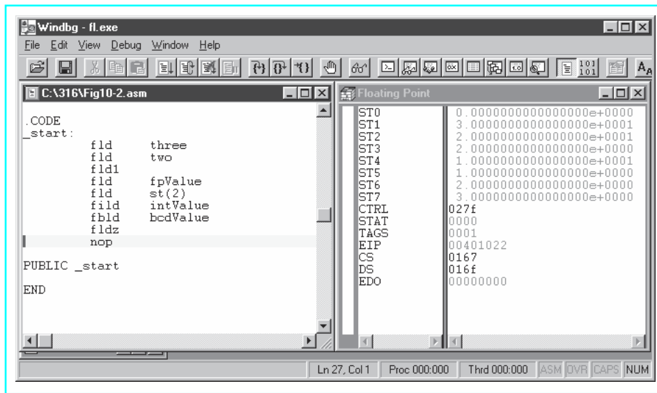
Figure 10.2 Windbg view of floating point execution
