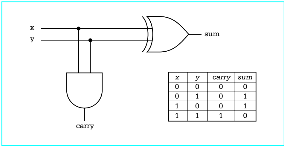
Figure 8.11 Half adder circuit
