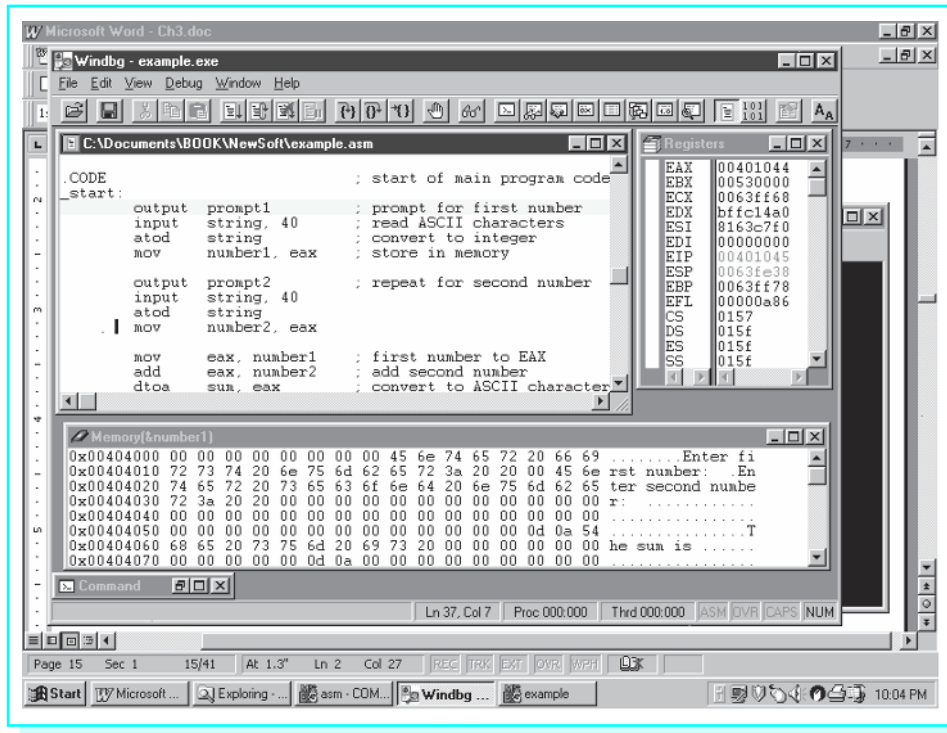
Figure 3.4 Windbg ready for tracing a program
