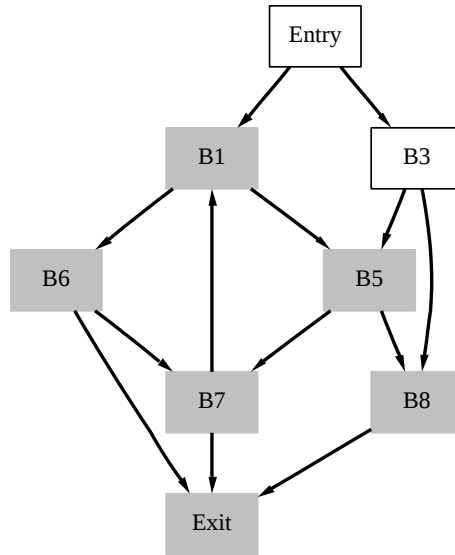
Figure 4.4 Vertices reachable from block B_1 .
