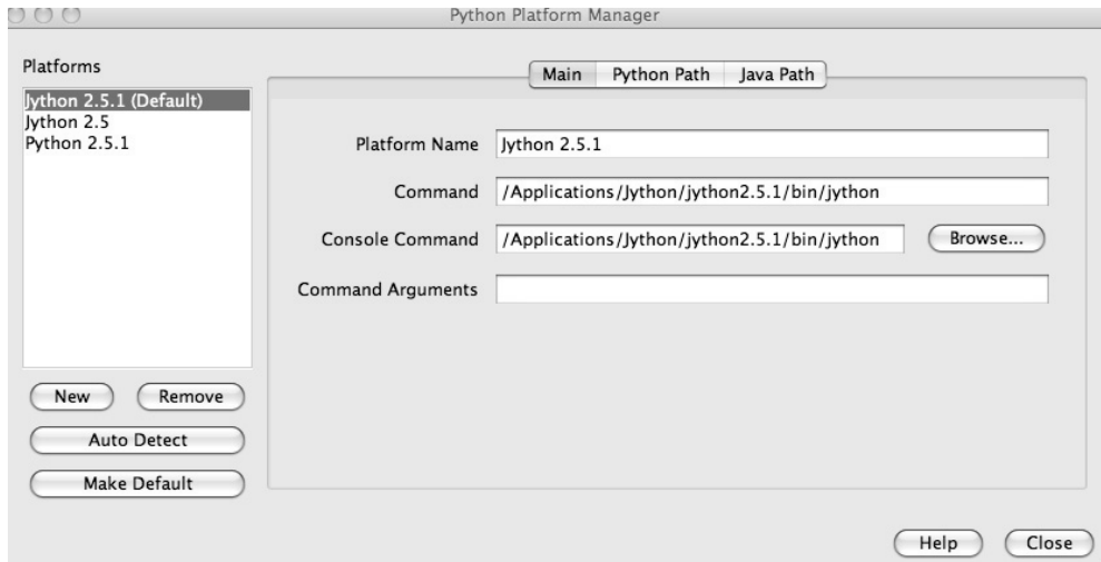
Figure 11-7. Adding your Jython installation as a platform option and making it the default
