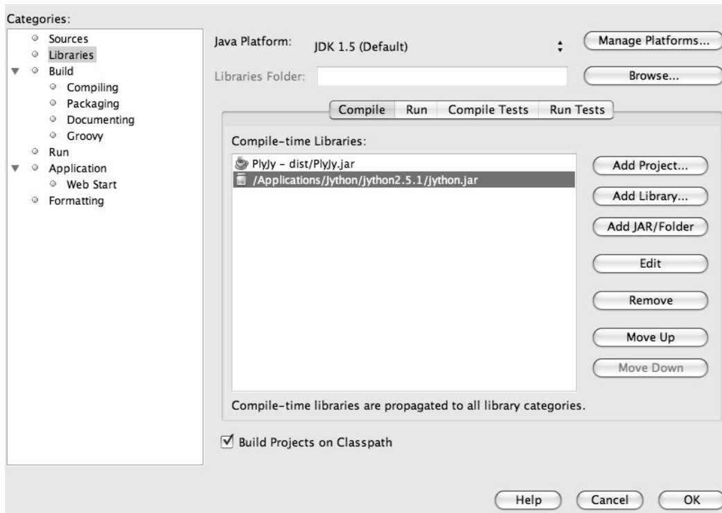
Figure 11-9. Adding the JAR file
