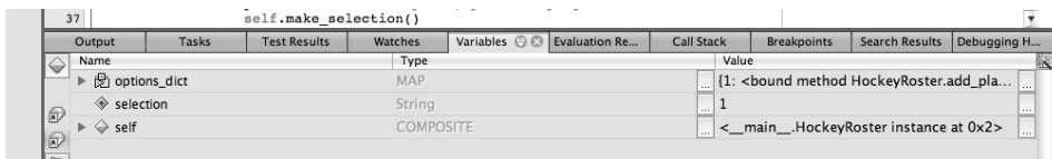
Figure 11-15. The values of all local variables at this current point in the program
