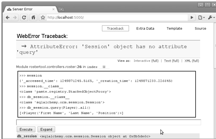
Figure 15-2. Error message caused by use of Session
