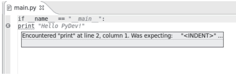
Figure 11-3. Error explanation appears when you hover over the error mark.
