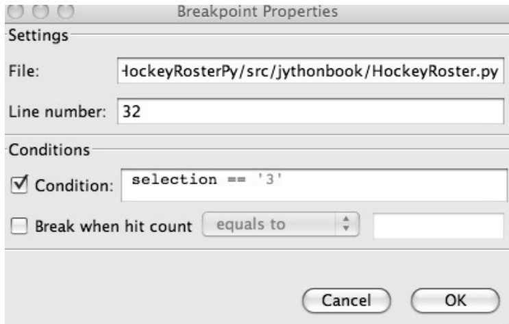
Figure 11-17. Setting a condition for halting the debugger
