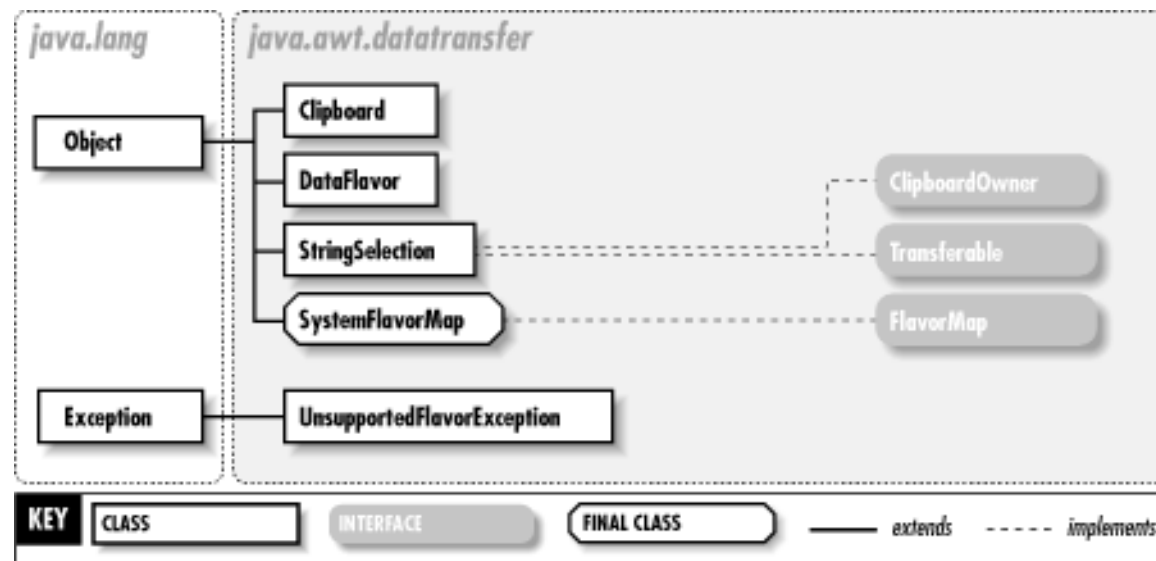
Figure 11-1. The java.awt.datatransfer package
