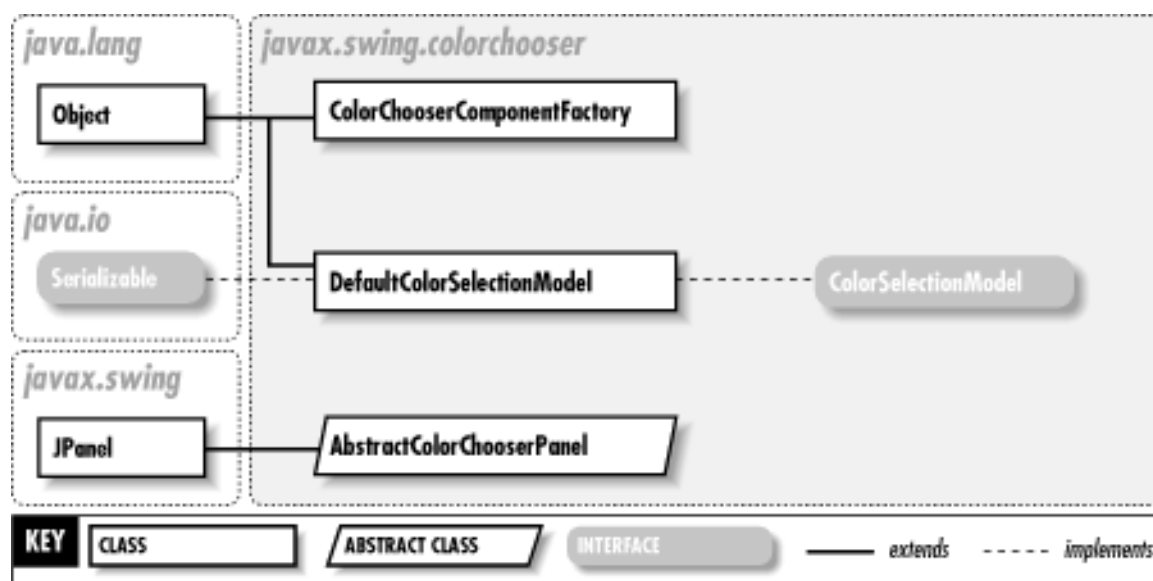
Figure 25-1. The javax.swing.colorchooser package
