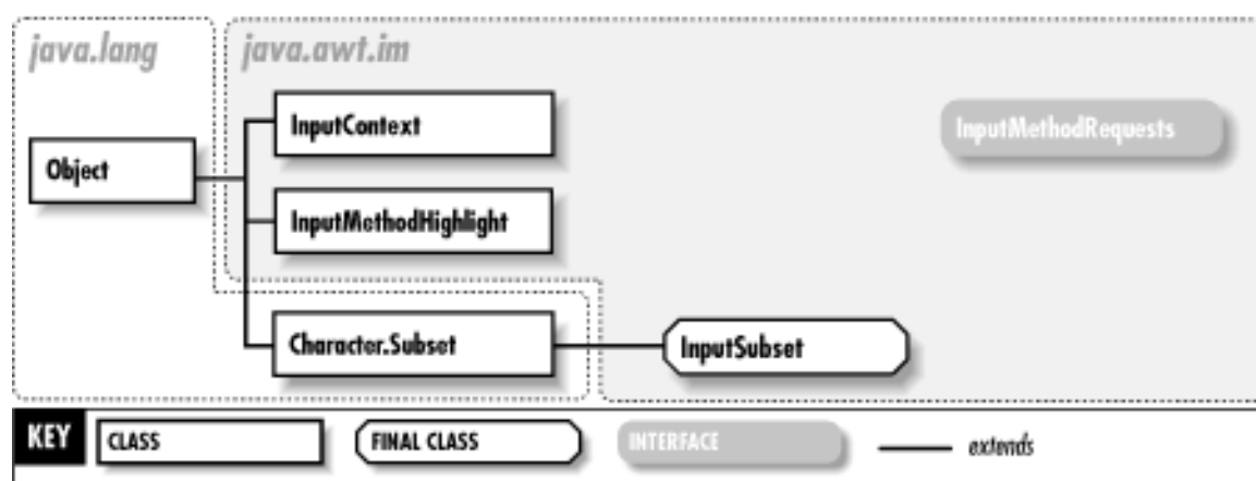
Figure 17-1. The java.awt.im package
