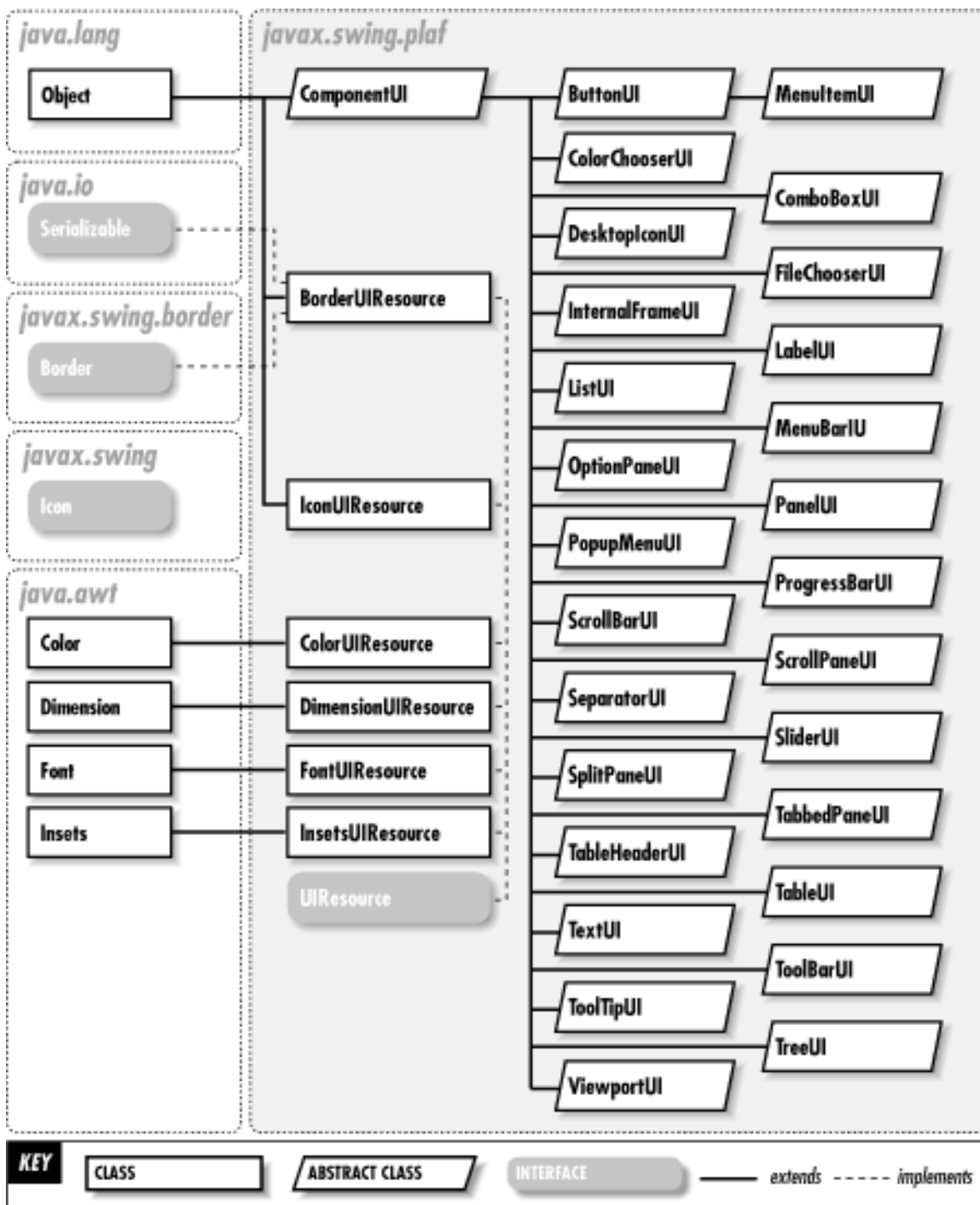
Figure 28-1. The javax.swing.plaf package
