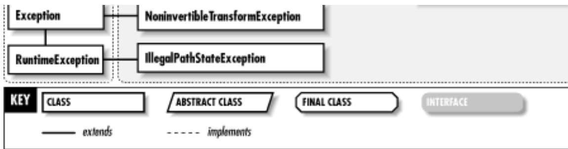
Figure 16-1. The java.awt.geom package
