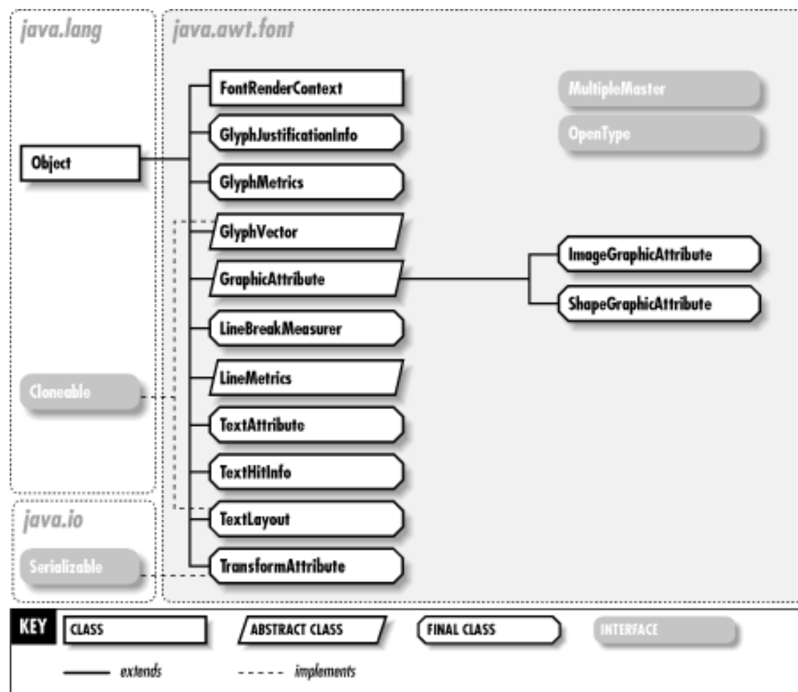
Figure 15-1. The java.awt.font package
