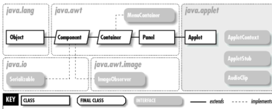
Figure 8-1. The java.applet package
