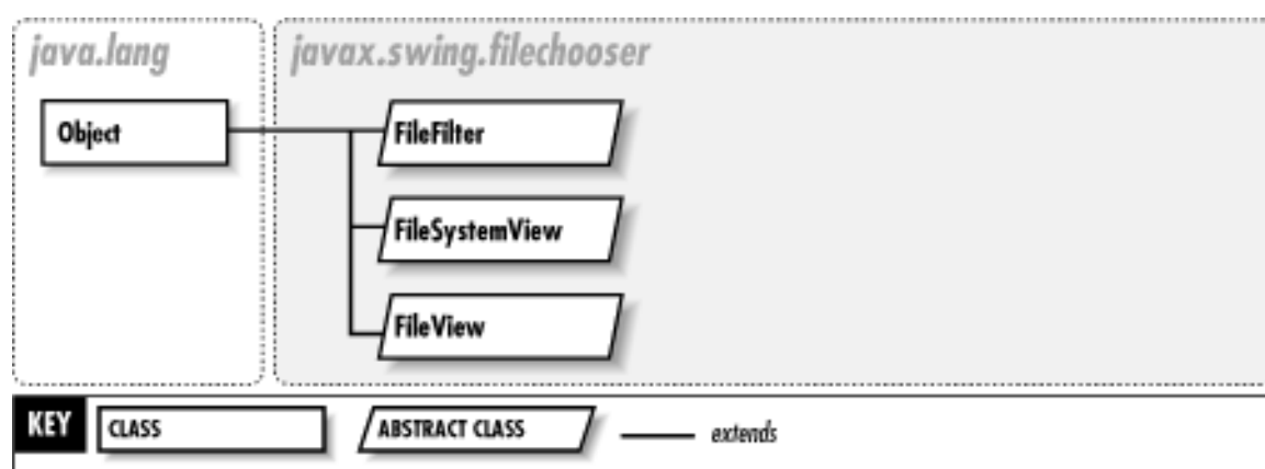
Figure 27-1. The javax.swing.filechooser package
