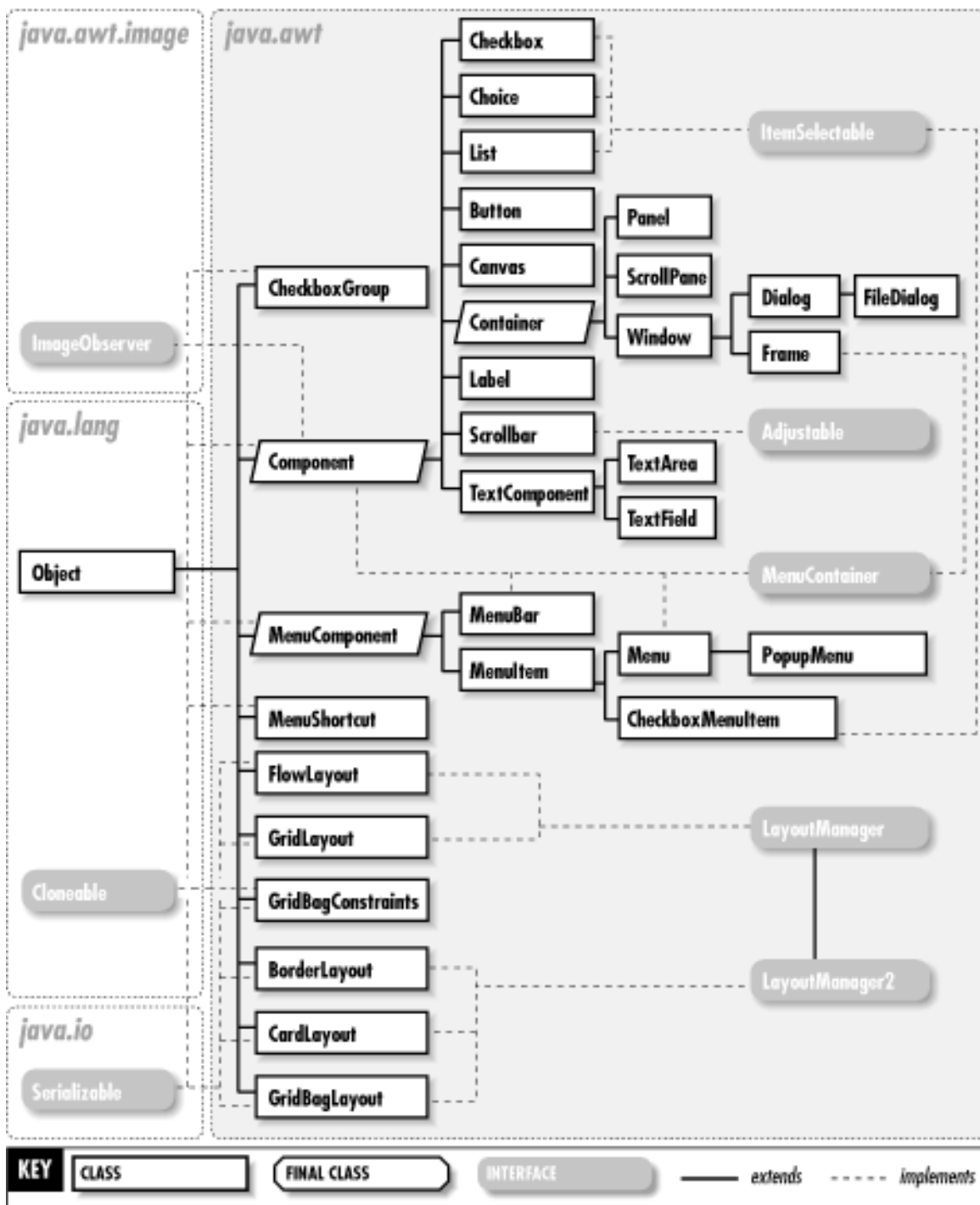
Figure 9-2. GUI classes of the java.awt package
