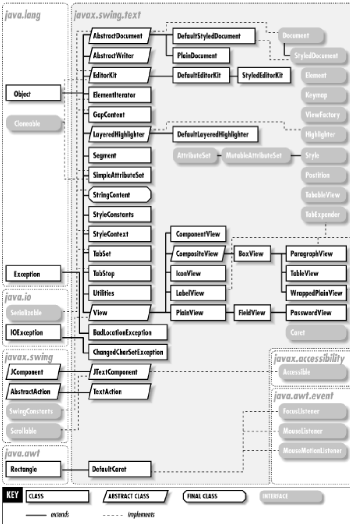
Figure 30-1. The javax.swing.text package
