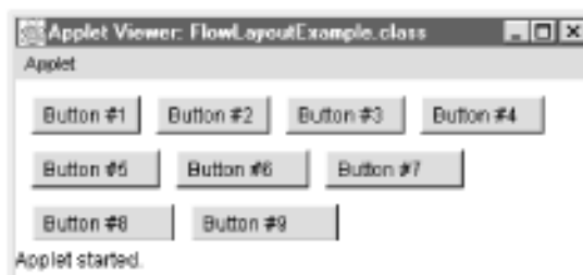
FlowLayout
