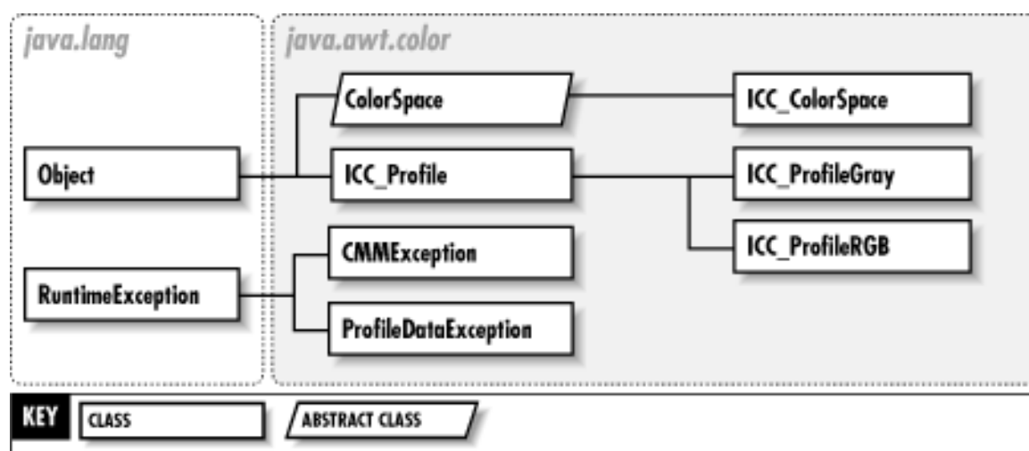
Figure 10-1. The java.awt.color package
