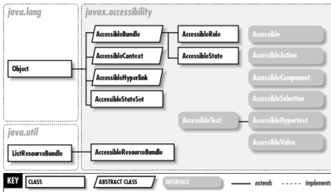
Figure 22-1. The javax.accessibility package
