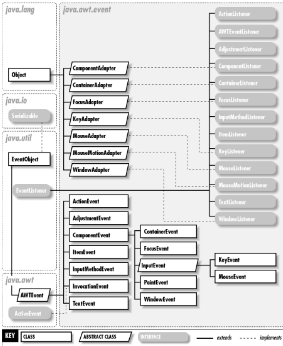
Figure 14-1. The java.awt.event package
