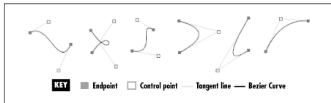
Figure 4-1. Bezier curves
