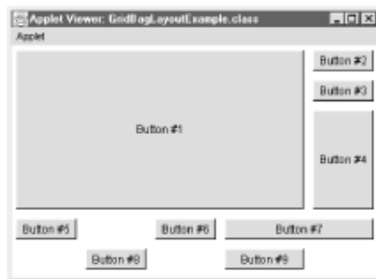
GridBagLayout
