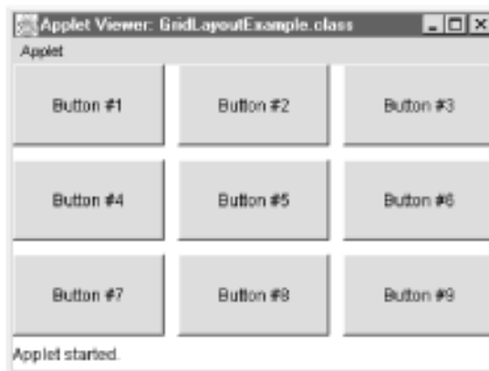
GridLayout
