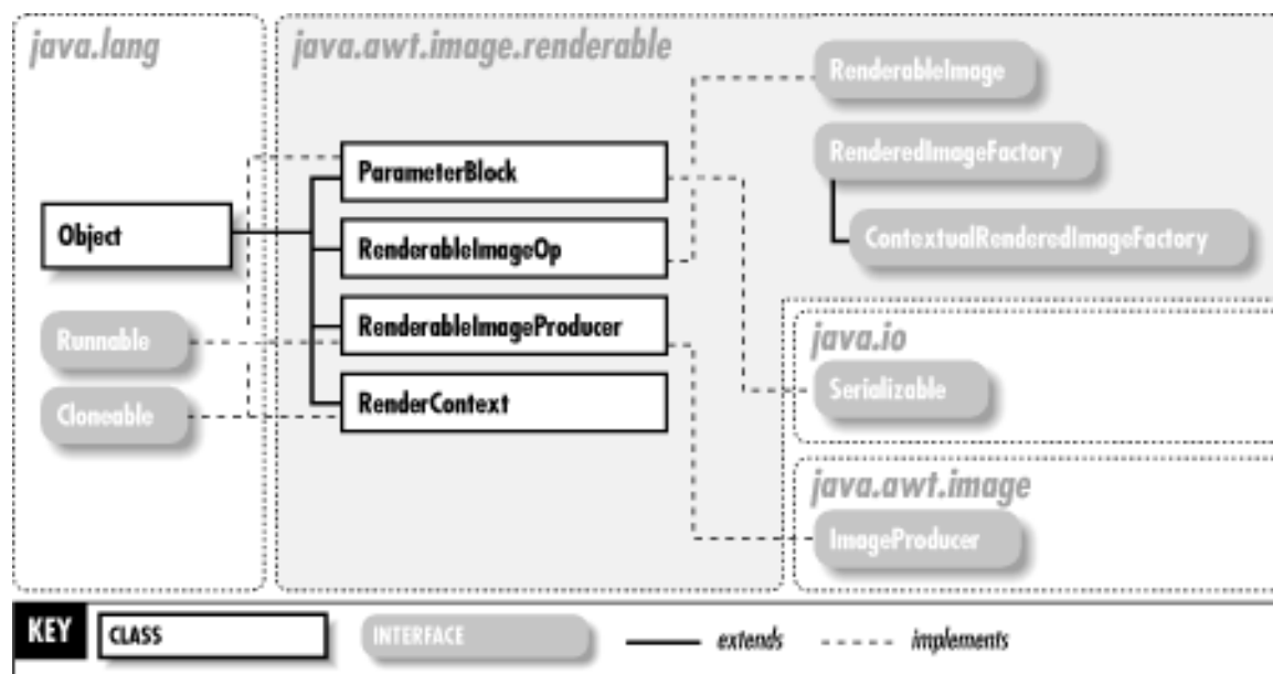
Figure 19-1. The java.awt.image.renderable package
