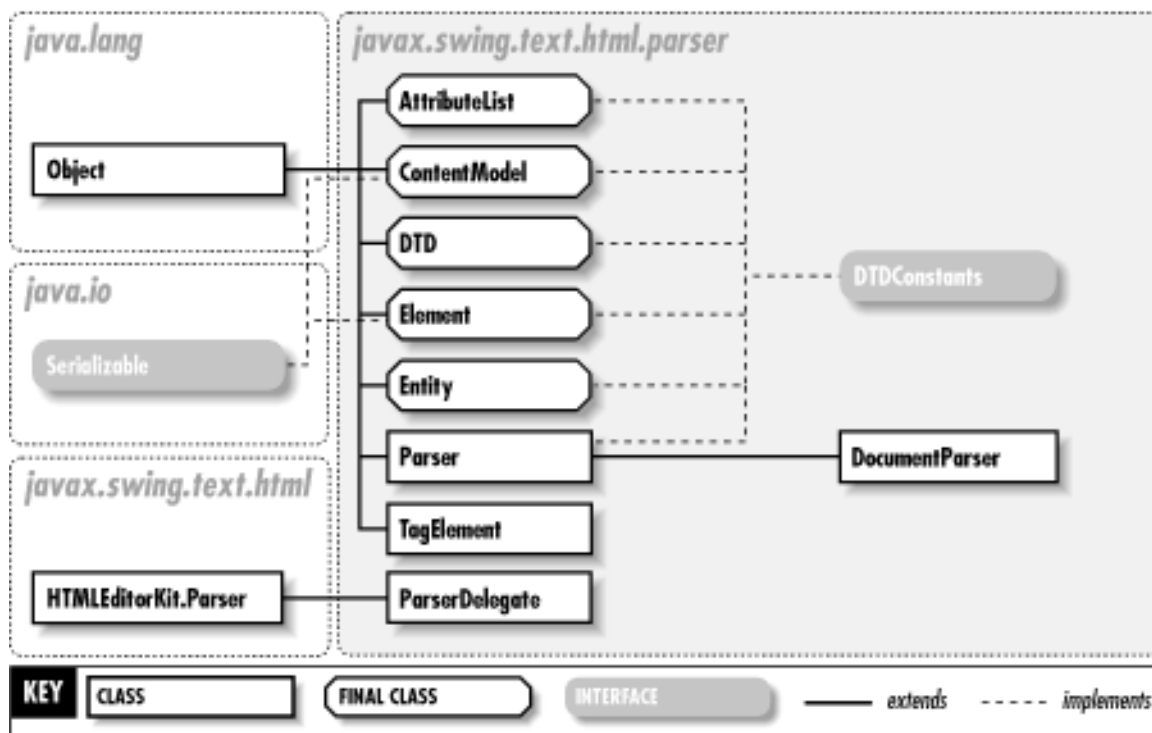
Figure 32-1. The javax.swing.text.html.parser package
