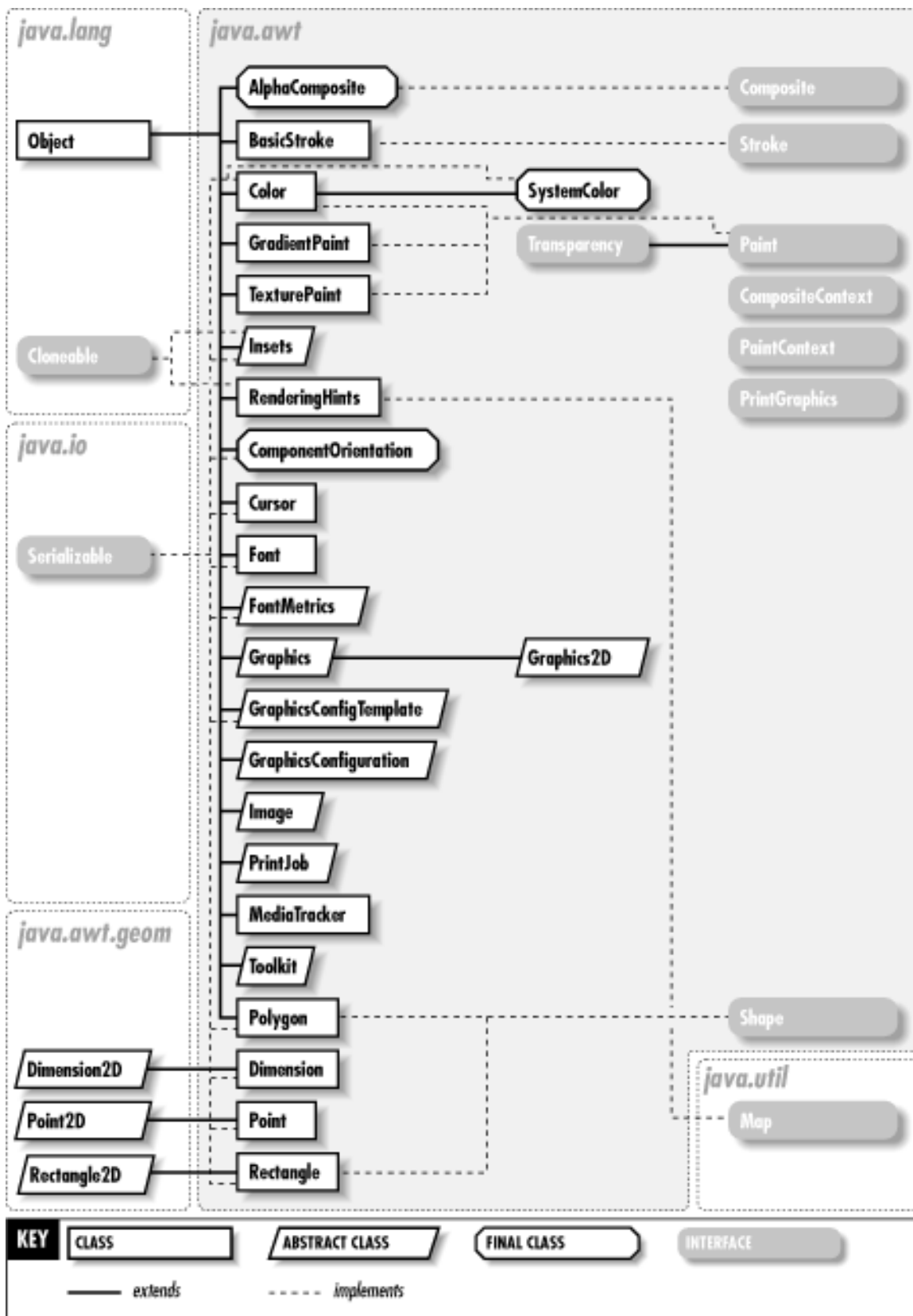
Figure 9-1. Graphics classes of the java.awt package
