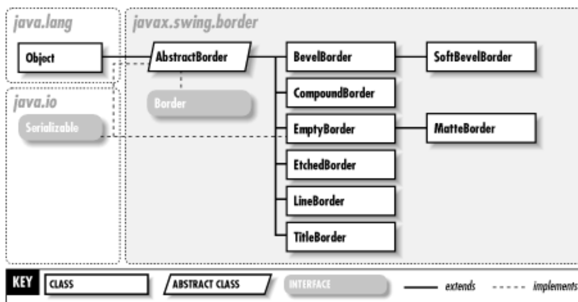
Figure 24-1. The javax.swing.border package
