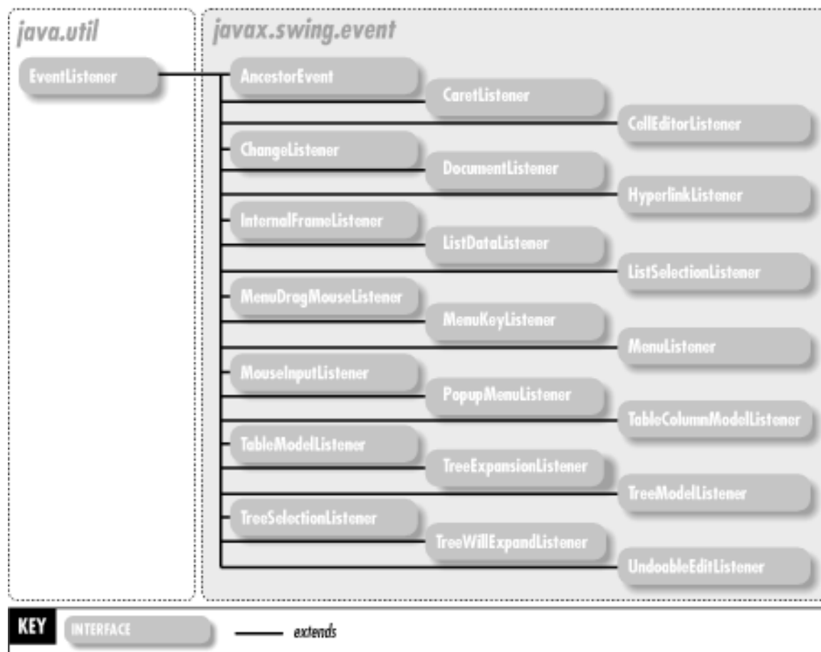
Figure 26-2. The event listeners of the javax.swing.event package
