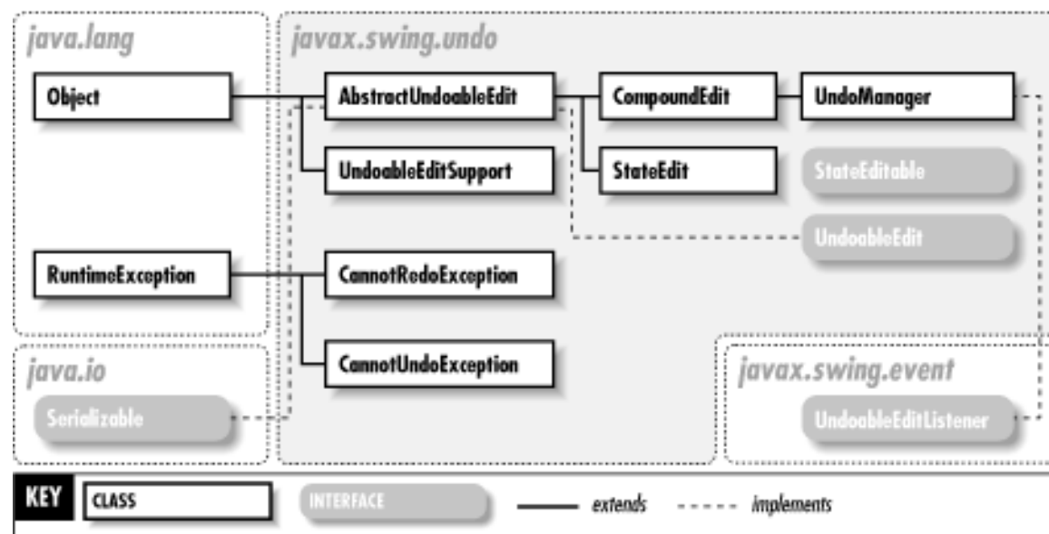
Figure 35-1. The javax.swing.undo package
