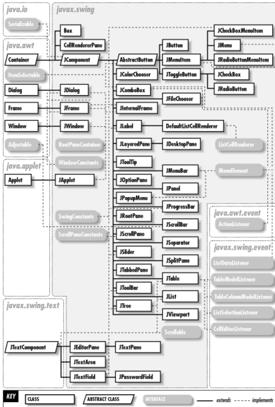
Figure 23-1. Components of the javax.swing package
