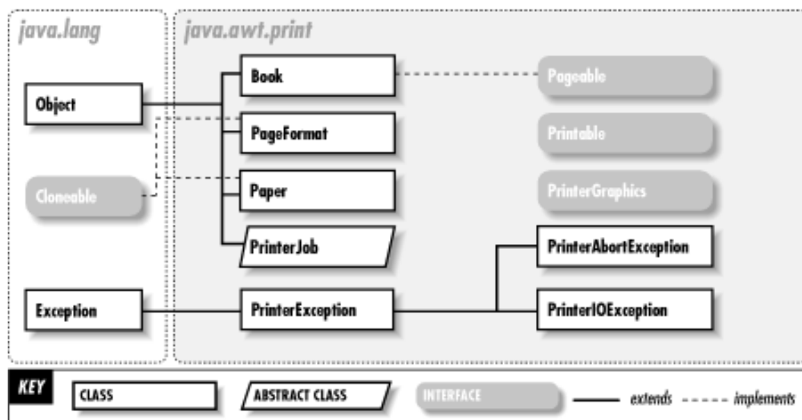
Figure 21-1. The java.awt.print package
