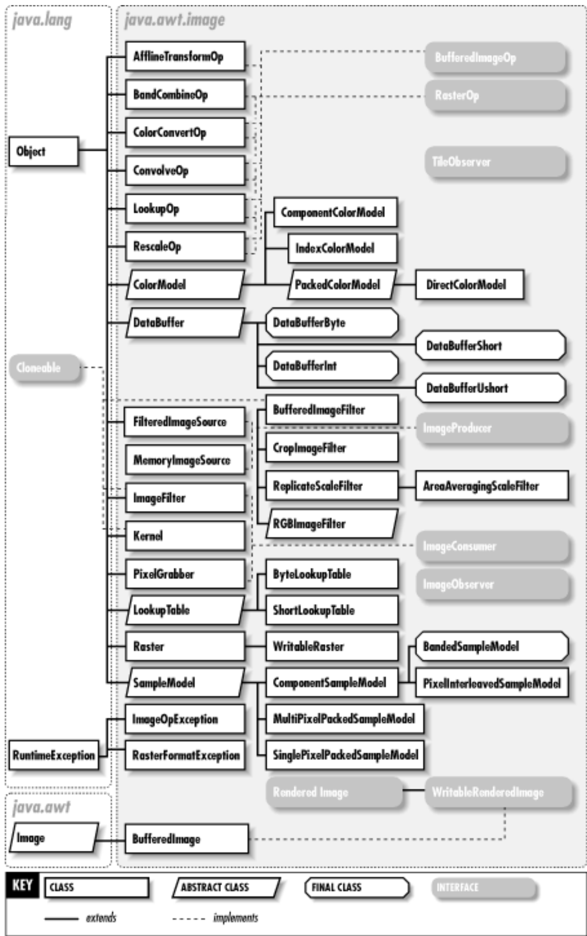
Figure 18-1. The java.awt.image package
