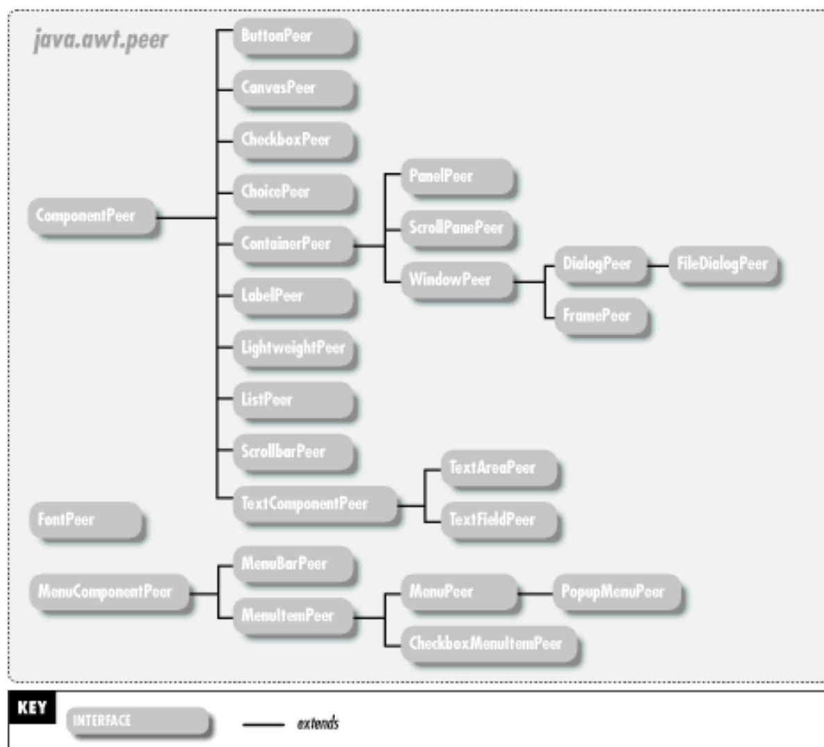
Figure 20-1. The java.awt.peer package
