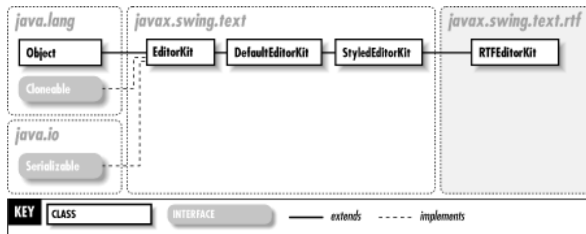
Figure 33-1. The javax.swing.text.rtf package
