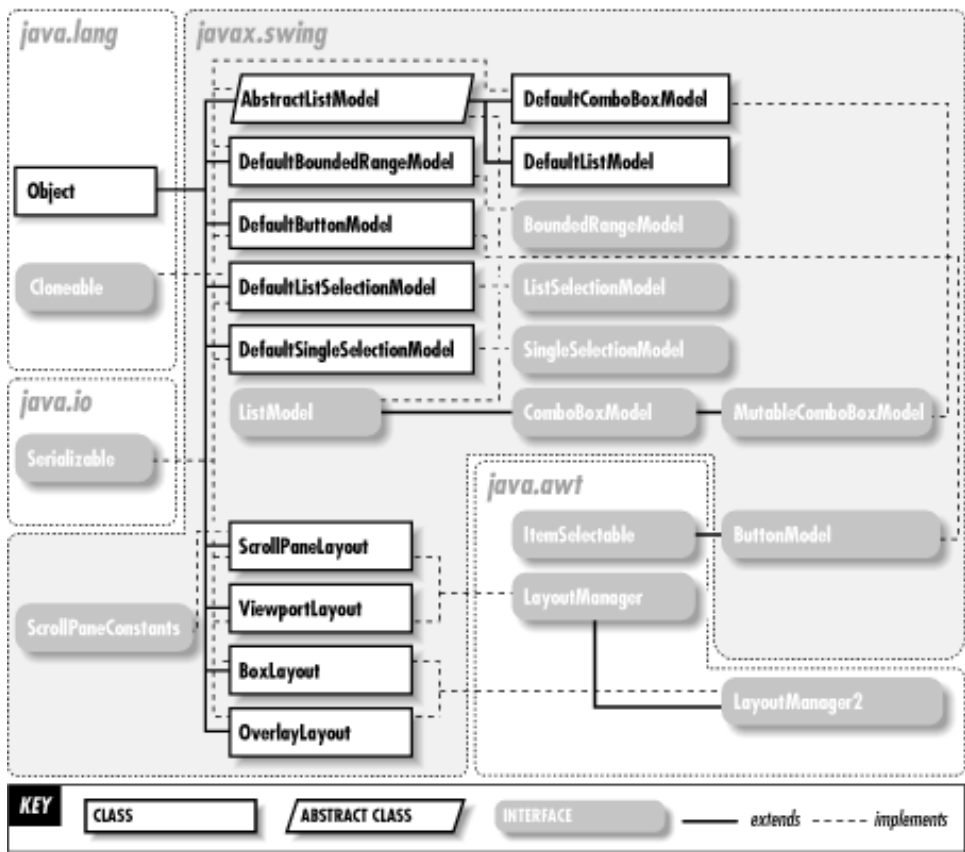
Figure 23-2. Models and layout managers of the java.swing package
