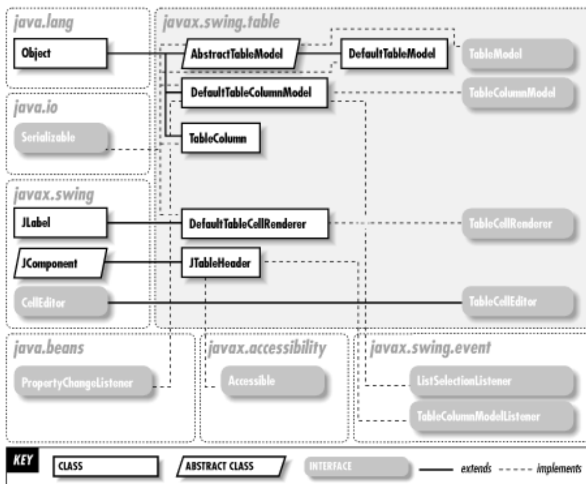
Figure 29-1. The javax.swing.table package
