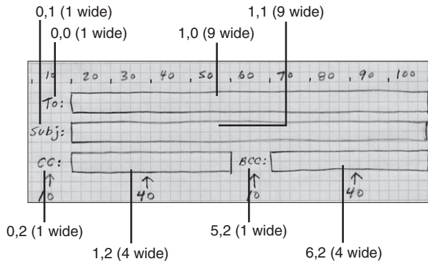
FIGURE 11.7 Choosing cells for components in the grid.
