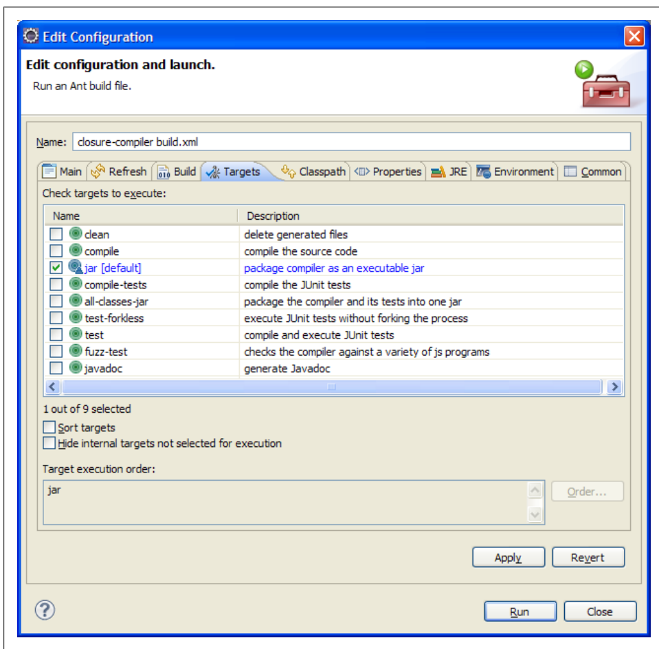
Figure 14-3. Ant dialog in Eclipse.
