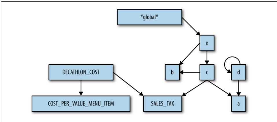
Figure 13-1. Dependency graph.
