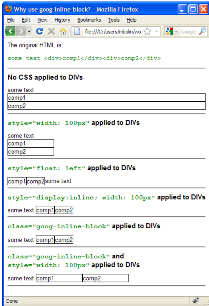
Figure 8-9. Using goog-inline-block to place elements side by side.
