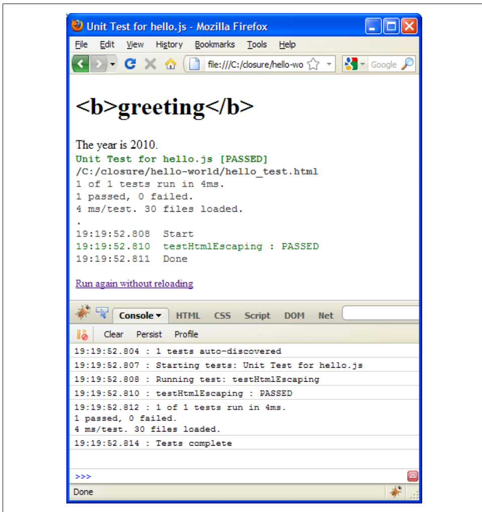
Figure 1-5. Test results for hello_test.html .
