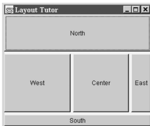
Figure 14-29. Layout4.py Result
