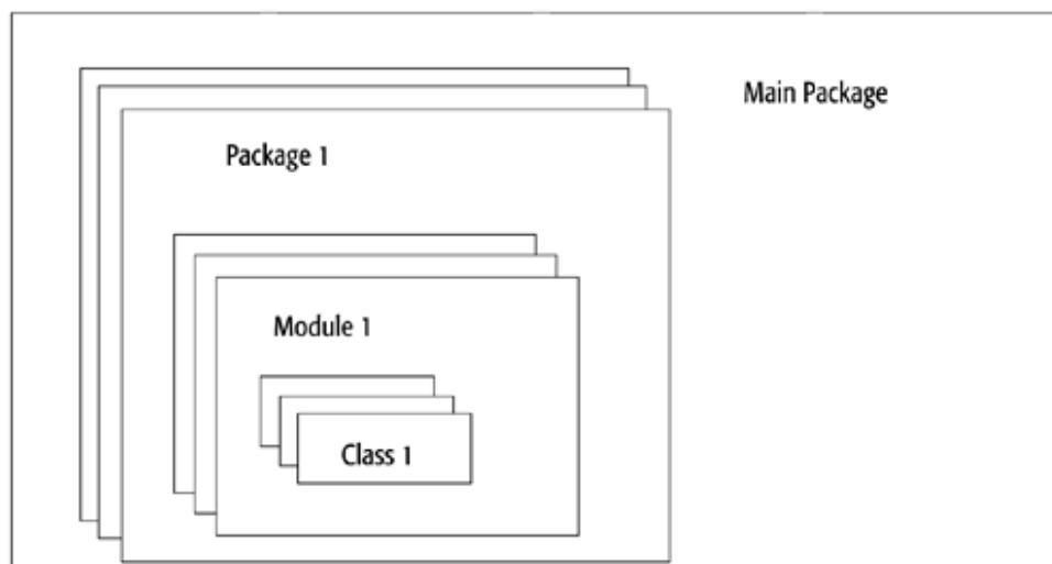
Figure 5-1. Program Organization
