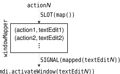
Figure 9.10 The MDI Editor’s signal mapper
