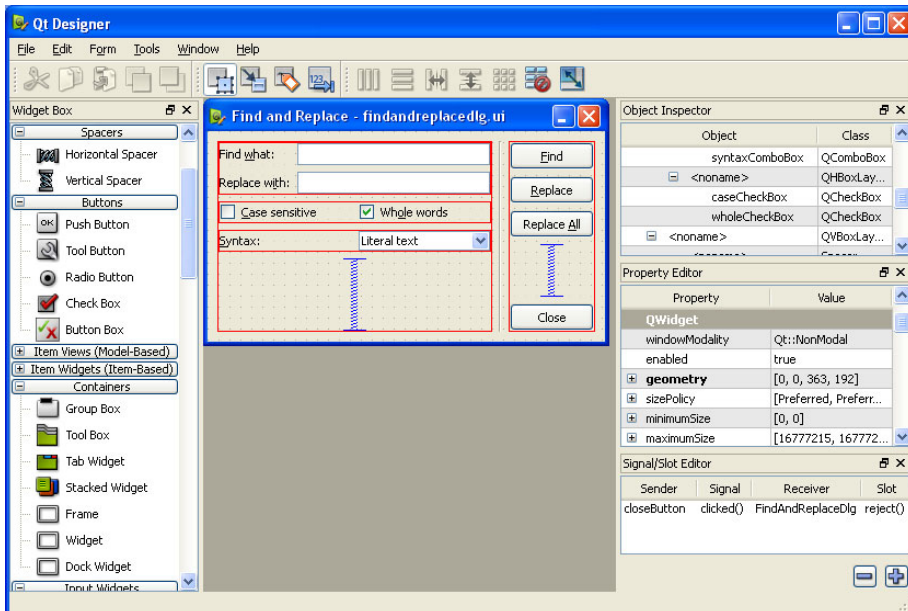
Figure 7.1 Qt Designer
