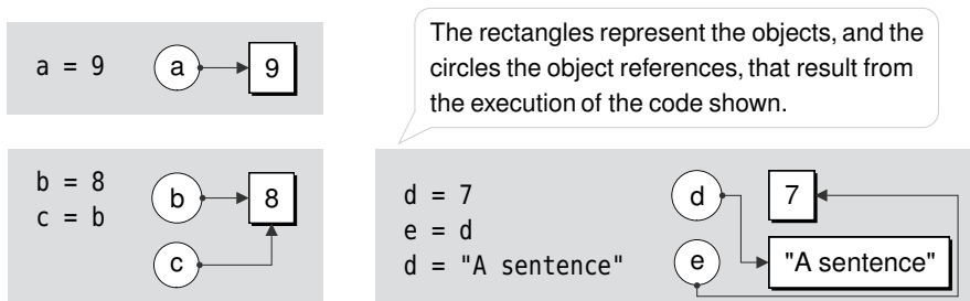
Figure 1.2 Object references and objects
