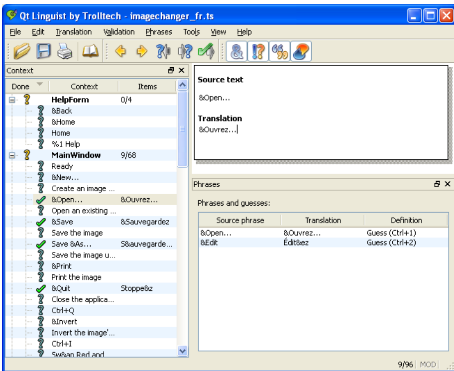
Figure 17.2 Qt Linguist
