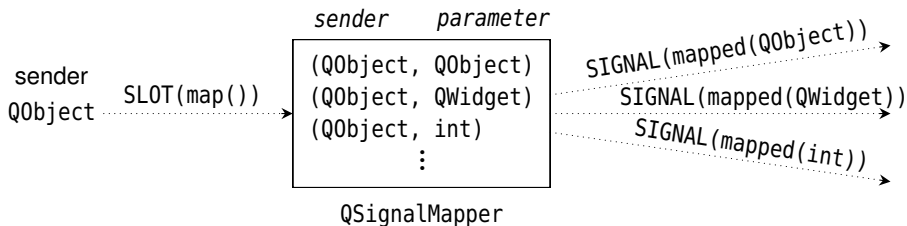
Figure 9.9 The general operation of a QSignalMapper
