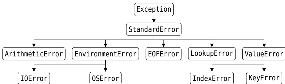
Figure 2.1 Some of Python's exception hierarchy
