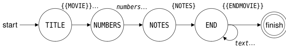
Figure 8.5 The My Movies text format's finite state automaton for each movie
