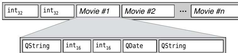
Figure 8.3 The QDataStream My Movies file format
