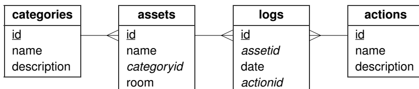
Figure 15.4 The Asset Manager database design
