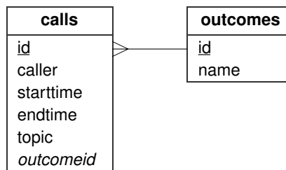
Figure 15.1 The Phone Log database design
