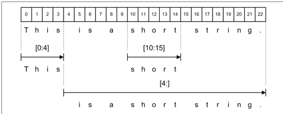
Figure 3-3. String indexing
