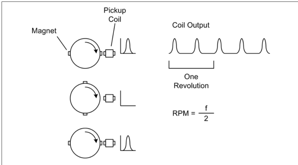
Figure 2-22. Electromagnetic tachometer
