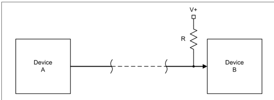
Figure 2-28. Signal pull-up
