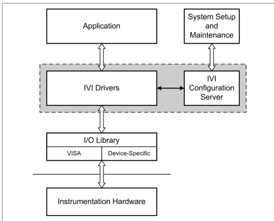
Figure 11-3. IVI architecture overview
