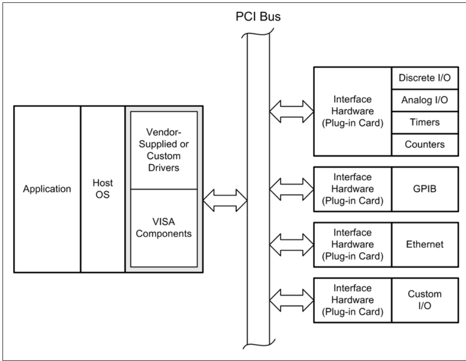
Figure 7-43. PCI interface cards
