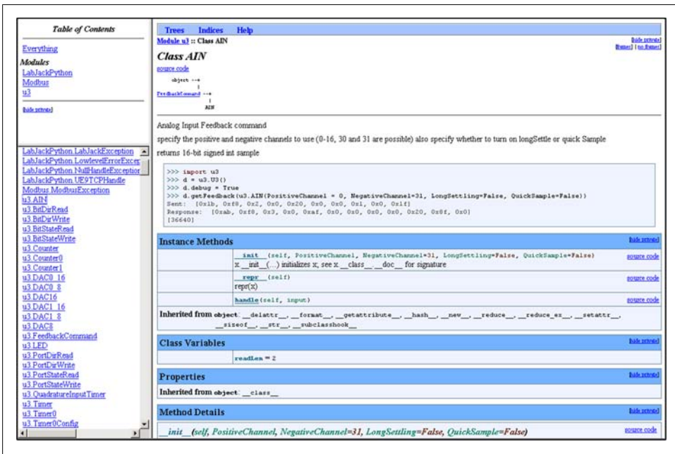
Figure 14-10. Epydoc output for LabJackPython
