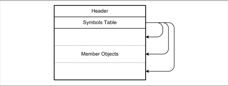
Figure 4-9. Generic library file internal format
