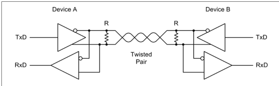
Figure 7-24. RS-485 interface drivers in two-wire mode
