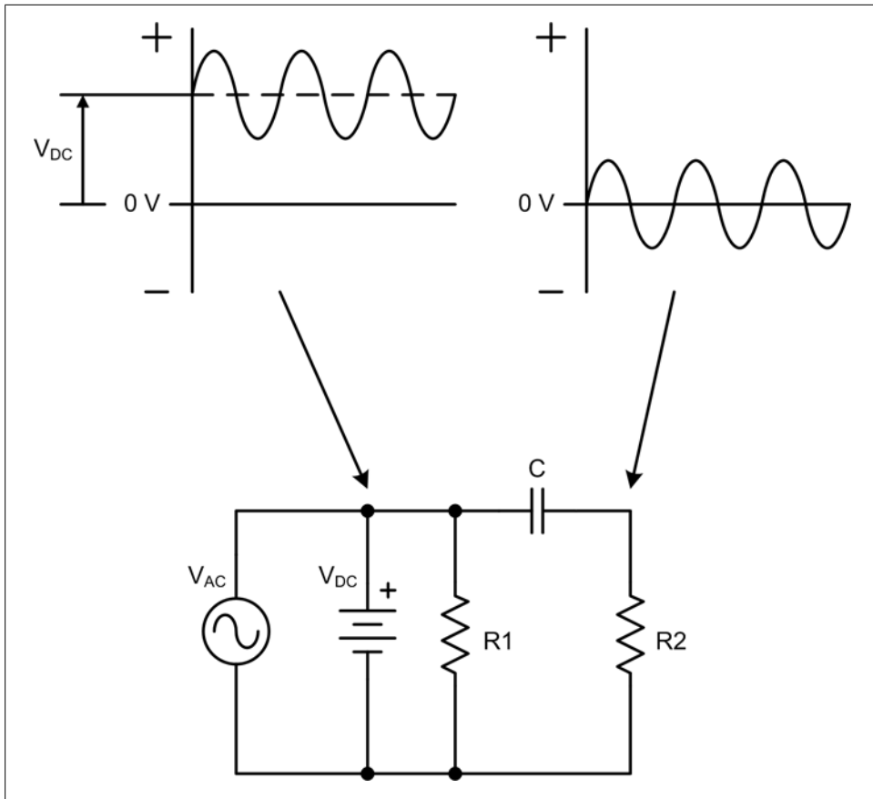
Figure 2-17. DC blocking
