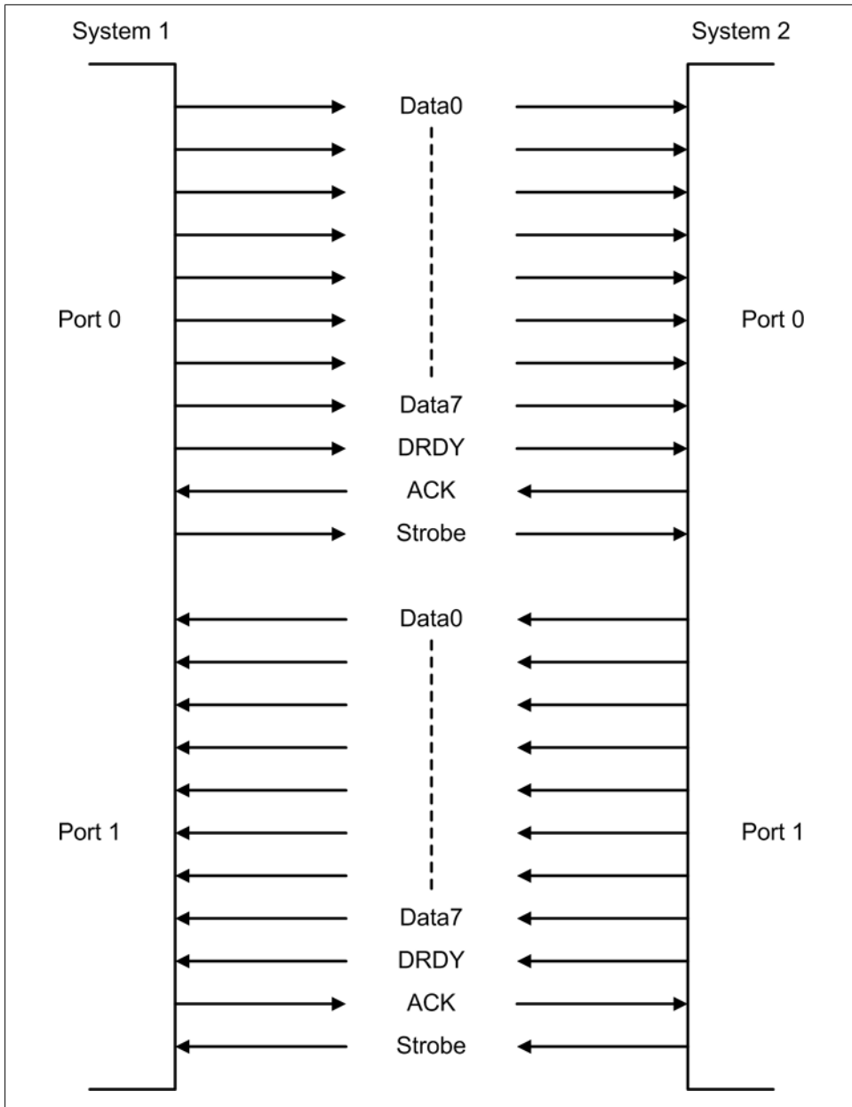
Figure 2-40. Bidirectional parallel interface
