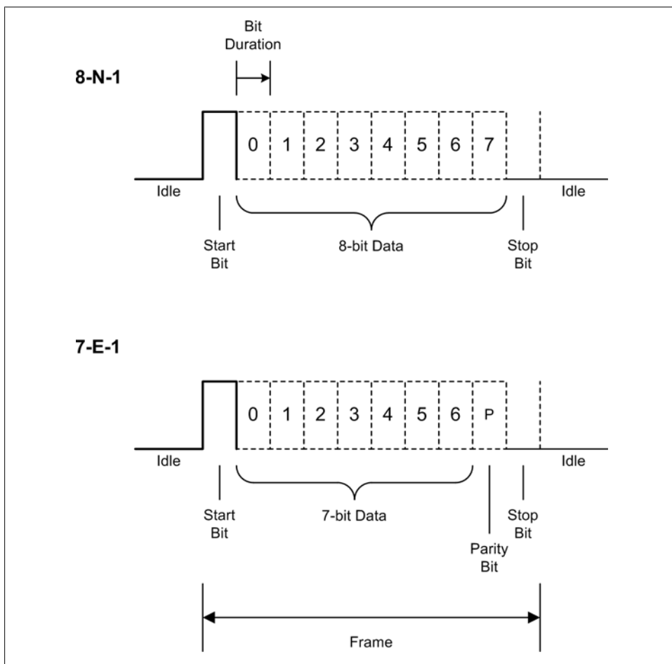
Figure 7-18. RS-232 data formats
