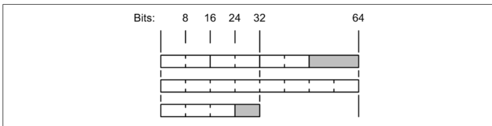
Figure 12-6. Structure padding
