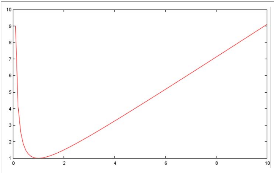
Figure 10-9. Plot of (x_0/(x_0^{**2}))+x_1
