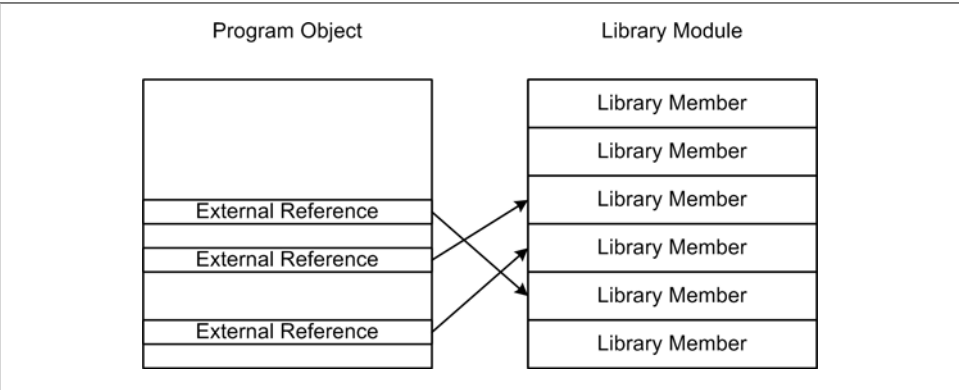
Figure 4-10. Program binary object linkage
