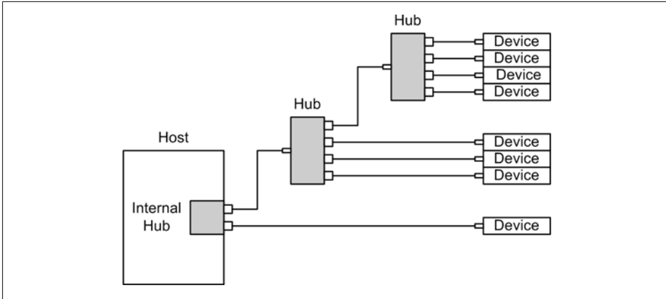
Figure 7-30. USB network
