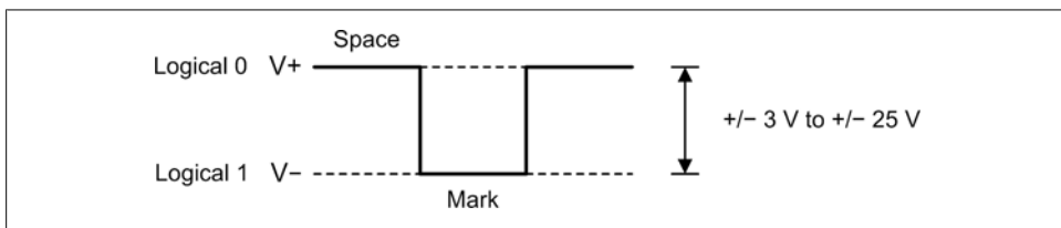
Figure 7-17. RS-232 signal levels
