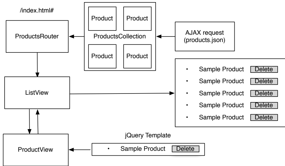
Figure 24—Listing Products with Backbone
