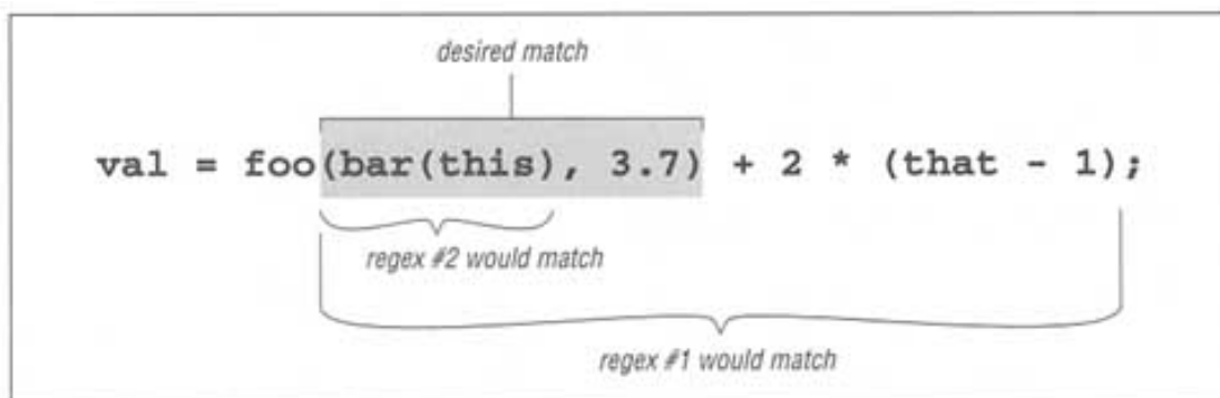
Figure 4-1: Match locations of our sample regexes
