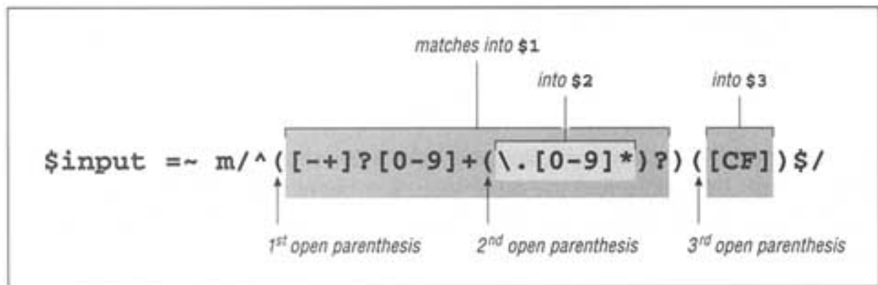
Figure 2-3: Nesting parentheses
